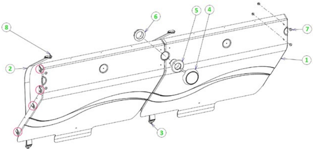
Figure 42 – Installing the pit wall and underwater light
